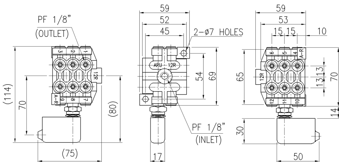
ARU-R-M (Limit switch option)
